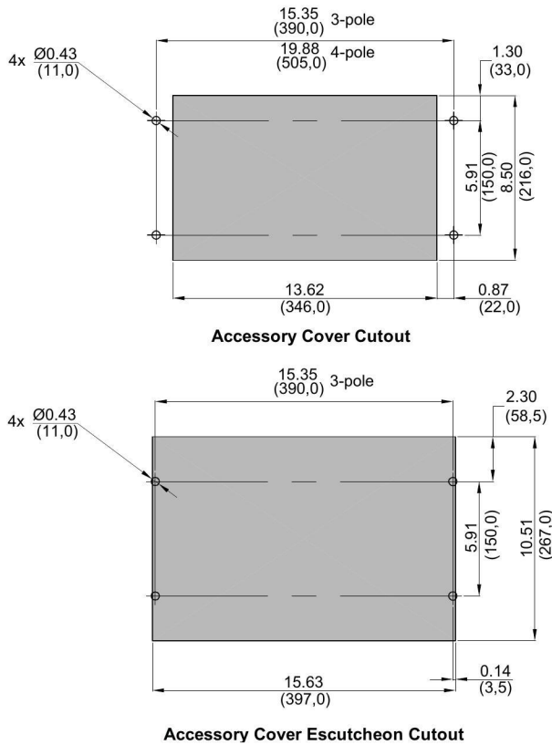
Figure 22: Mounting Hole and Enclosure Cover Cutouts Dimensions
